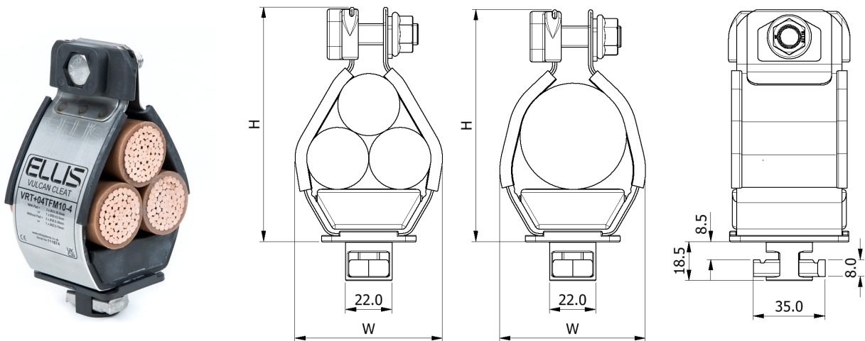
SINGLE FIX TWIST FOOT: VRT+00 TO VRT+12
