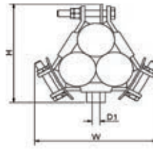
Single bolt base fixing
