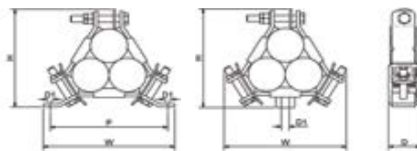
Two bolt base fixing
